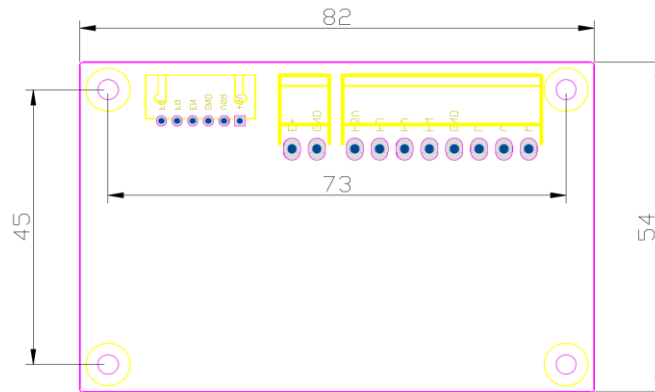
PCB尺寸图 (PCB DRAWING)
